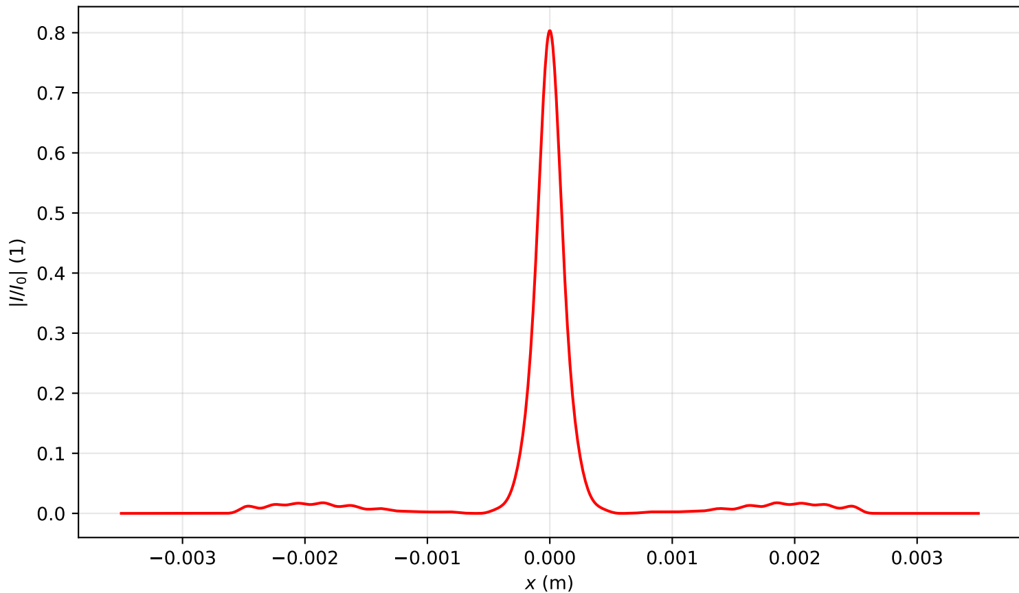
Intensity profile I(x, y = 0, z = 1.592)/I_0 , P_{in}=7.0P_{cr} , artificial time
